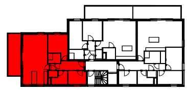
INPLANTINGSPLAN
